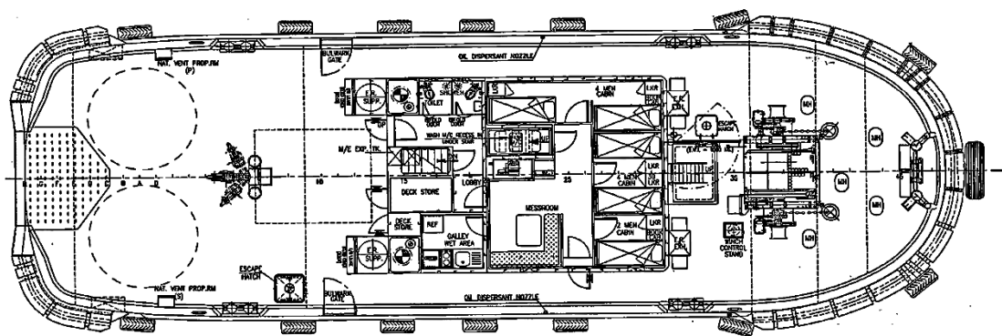
MAIN DECK
