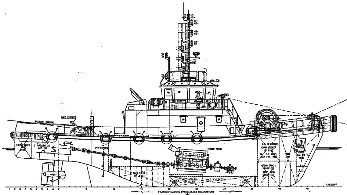
OUTBOARD PROFILE
