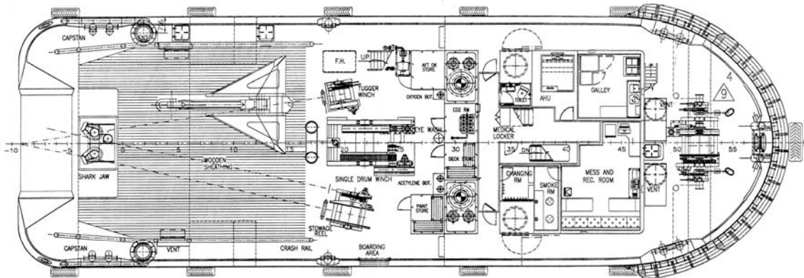
MAIN DECK
