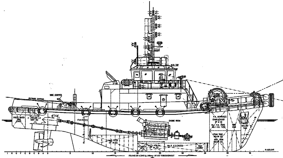
OUTBOARD PROFILE
